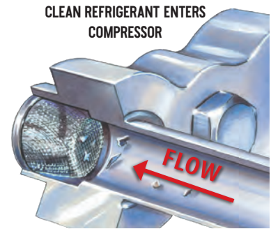
COMPRESSOR GUARD SCREEN PREVENTS DEBRIS ENTERING COMPRESSOR
